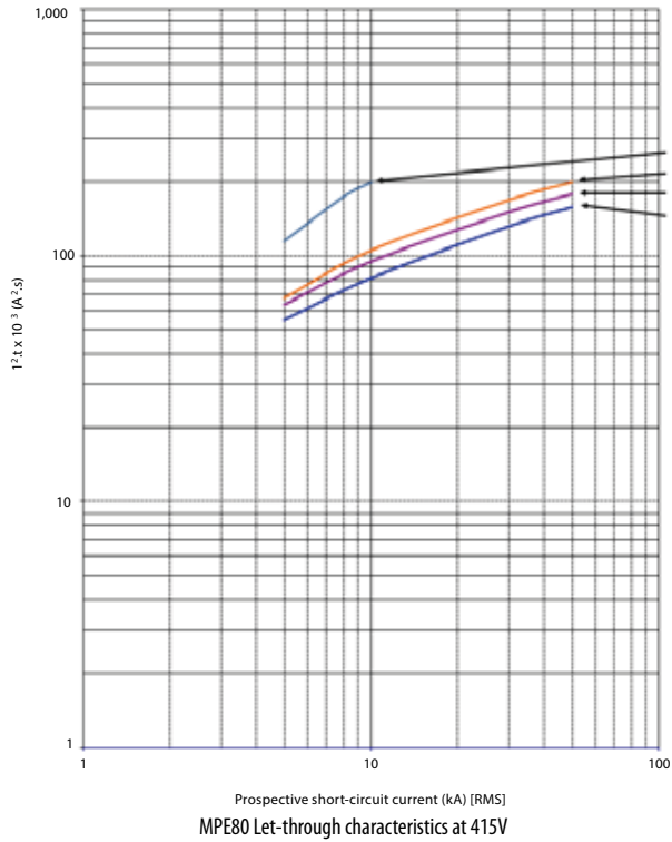
MPE80 Let-through characteristics at 415V
