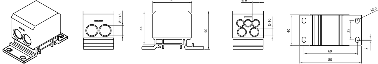
EDBS-50../EDBS-50../N, EDBS-50../PE
