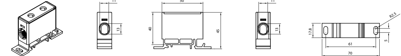
EDBS-50../EDBS-50../N, EDBS-50../PE
