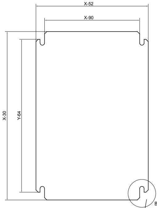
Mounting plate
